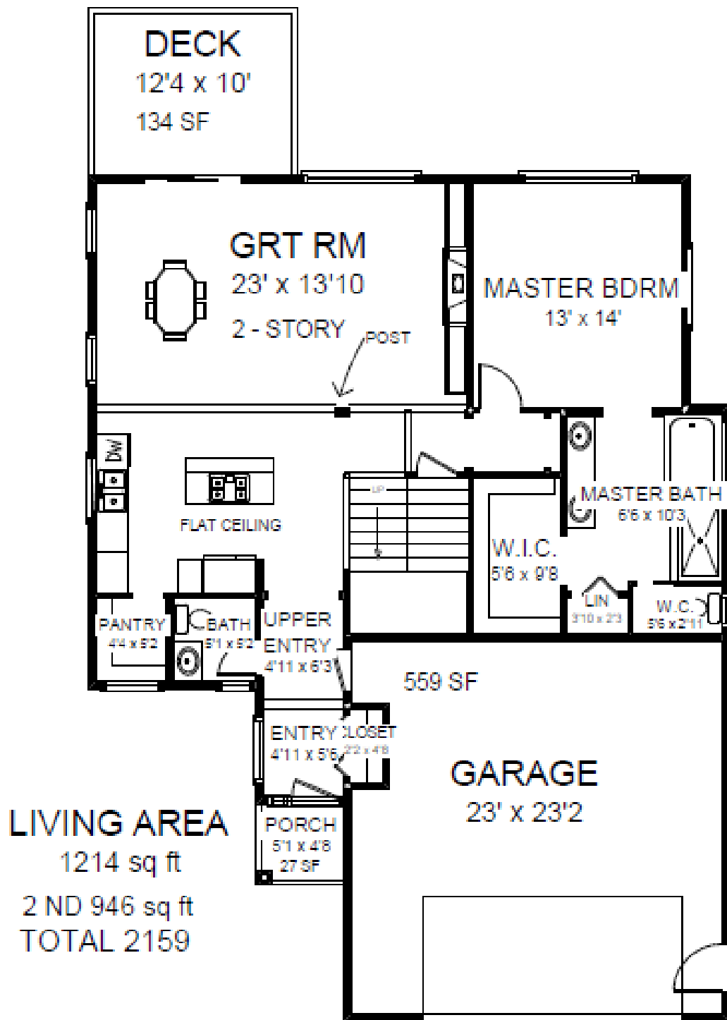
PLAN - 63 CLARISA
